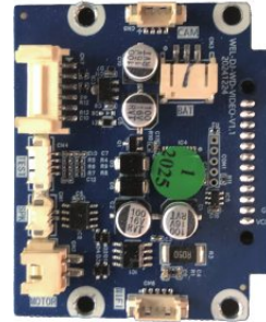
Mainboard 2
