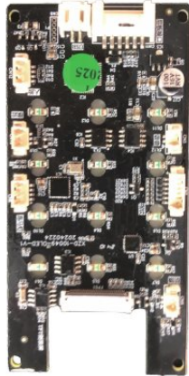
Mainboard 1
