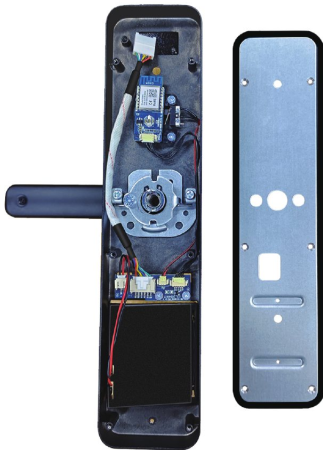
Back Panel
