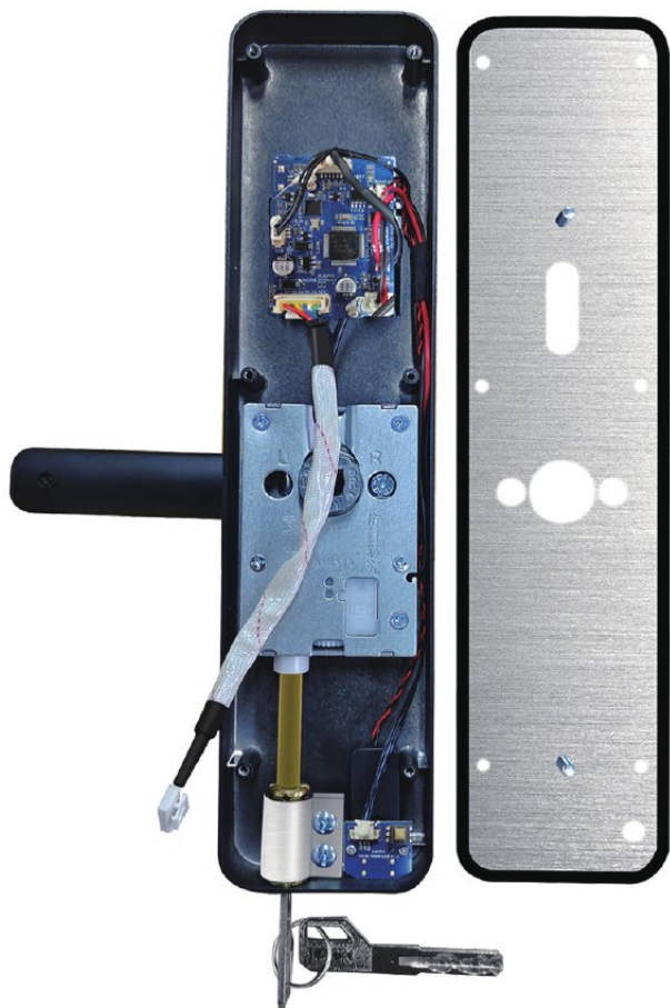
Front Panel
