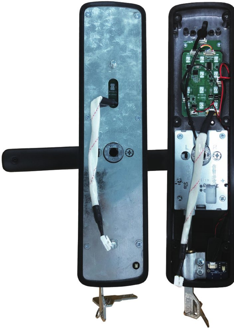
Front Panel
