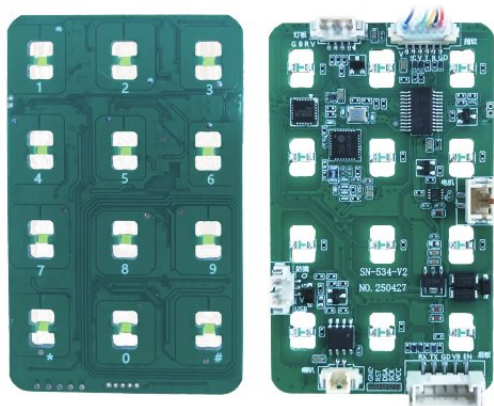
Mainboard 1
