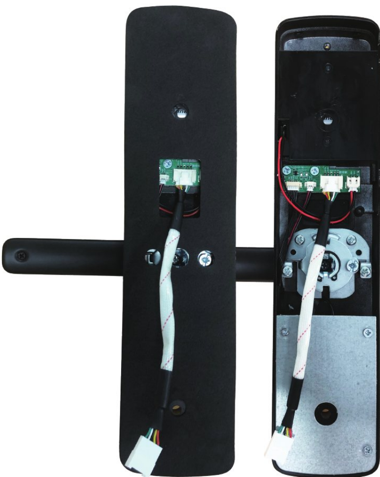
Back Panel
