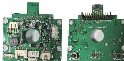
Mainboard 2
